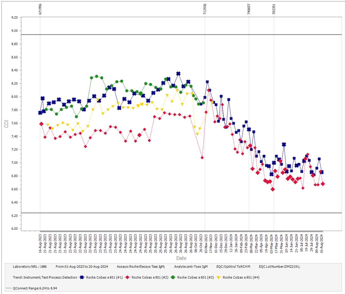
Figure 2 – Participant 1866 data demonstrating reagent lot trend observed for Optitrol ToRCH M DM22191 when testing with Roche Elecsys Toxo IgM by instrument.
